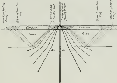
Fig. 98. Complete Diagram of Halation.
